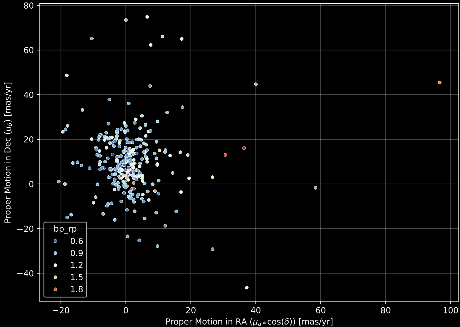
GALAH DR4 Field: [1056] Proper Motion Diagram (n= 298)
