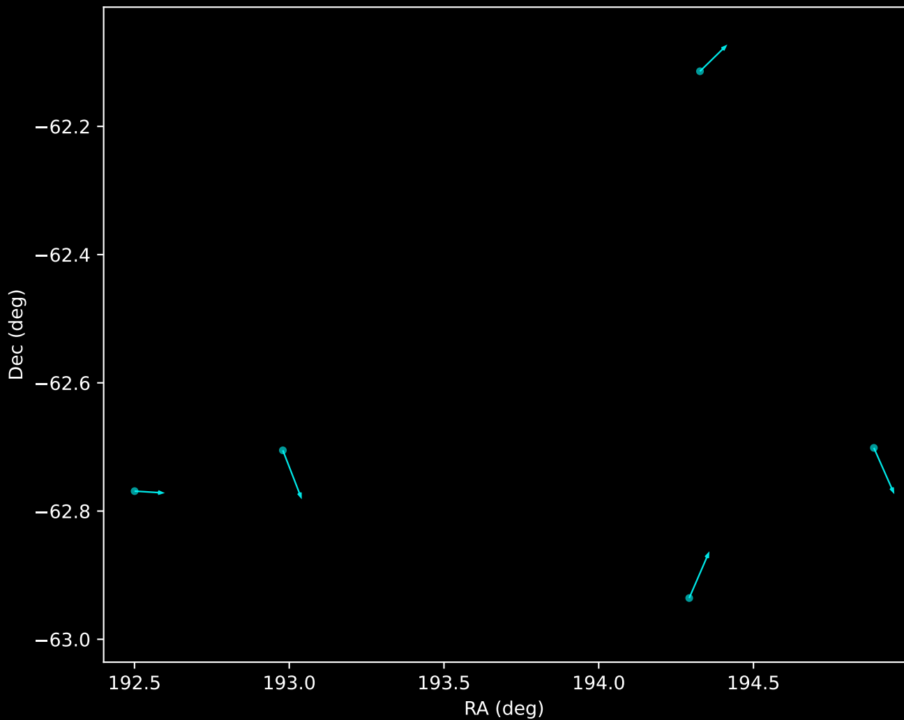
GALAH DR4 Noise Stream Proper Motion Vectors (n=5)
