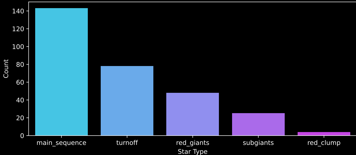
GALAH DR4 Field: [1056] Count plot of Star Type
