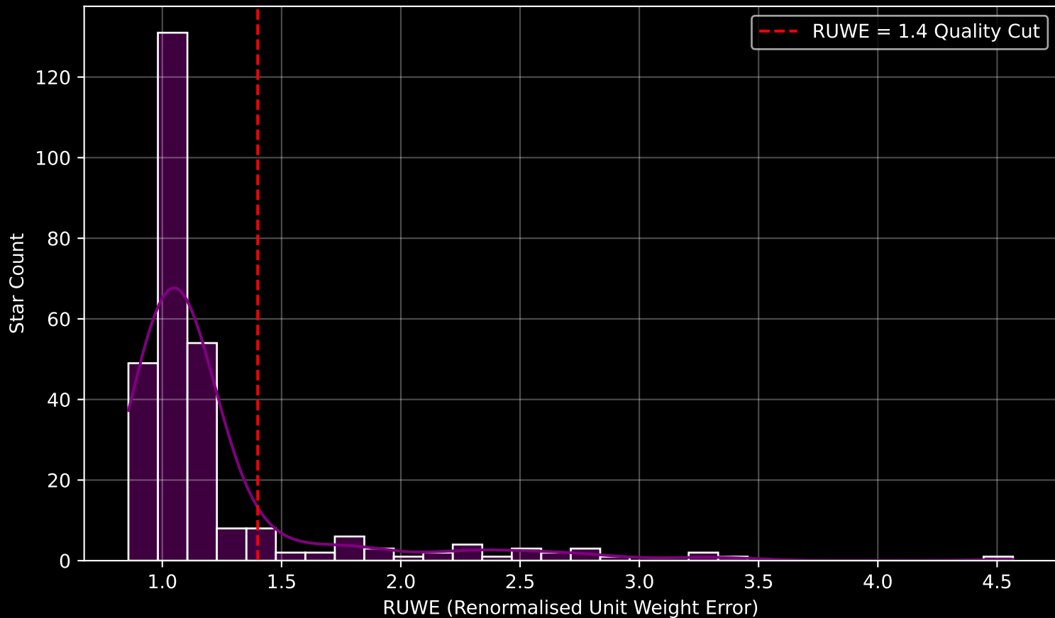
GALAH DR4 Field [1056] RUWE Distribution (n= 284)
